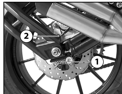
1. Rear sensor rotor 2. Rear wheel sensor
