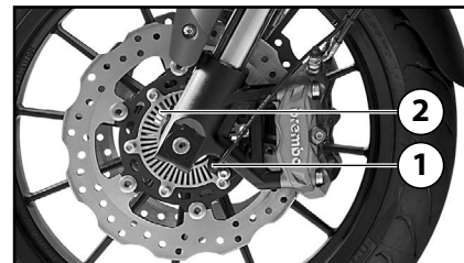
1. Front wheel sensor 2. Front sensor rotor
